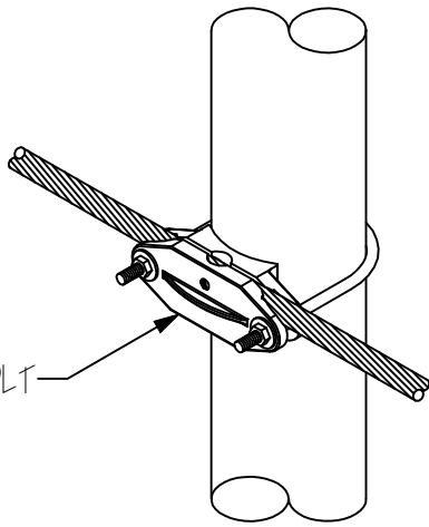
No.A804: Alum U-BOLT BONDING CLAMP
