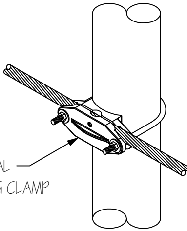
No. 805T: BIMETAL U-BOLT BONDING CLAMP
