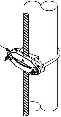
No. 805T: BIMETAL U-BOLT BONDING CLAMP
