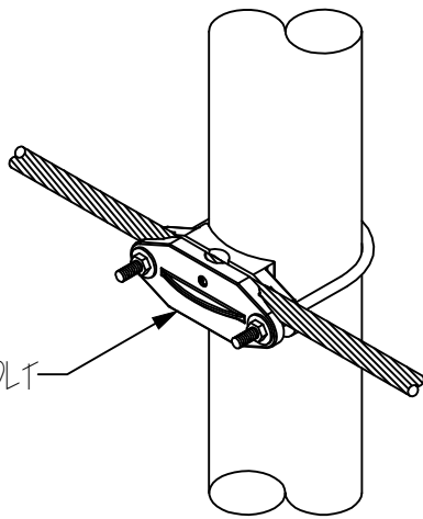
No.804: Cu U-BOLT BONDING CLAMP
