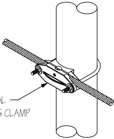
No. 803T: BIMETAL U-BOLT BONDING CLAMP
