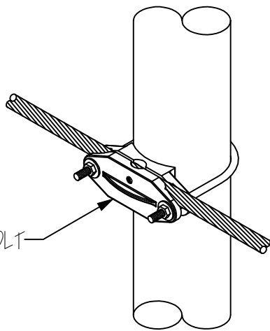
No.802: Cu U-BOLT BONDING CLAMP
