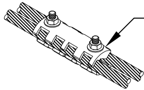
No. 424B: CAST BRONZE PARALLEL CABLE SPLICER
